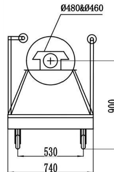
侧视图 LATERAL VIEW
